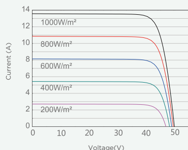
Current-Voltage Curve(SP540M-72H)
